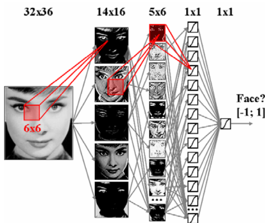
Fig. 2 – Convolutional neural network’s structure for the combined cascade of classifiers.
