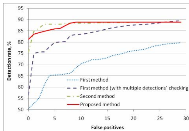
Fig. 4 – ROC-curves of the combined cascade of classifiers using different verification methods on CMU test set
